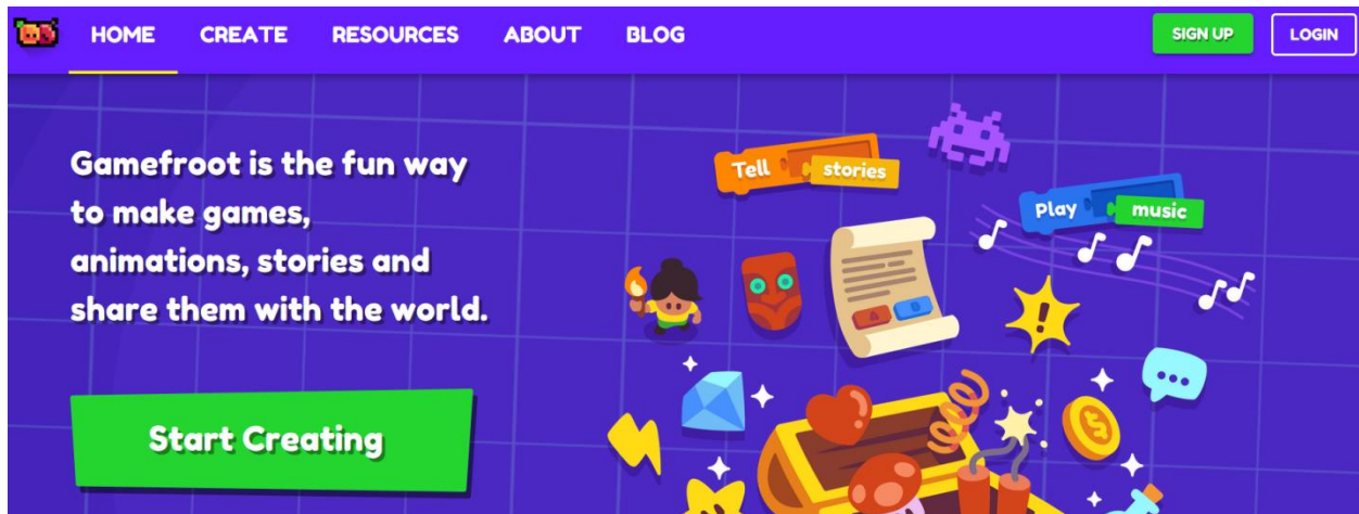
Figura 1 - Screenshot Gamefroot
